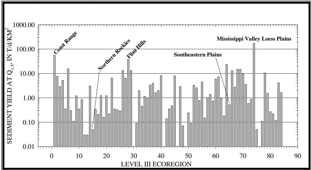
Figure 5. Comparison of national median suspended-sediment yields at the Q1.5 for 84 ecoregions of the continental United States (Simon et al., 2002c)
