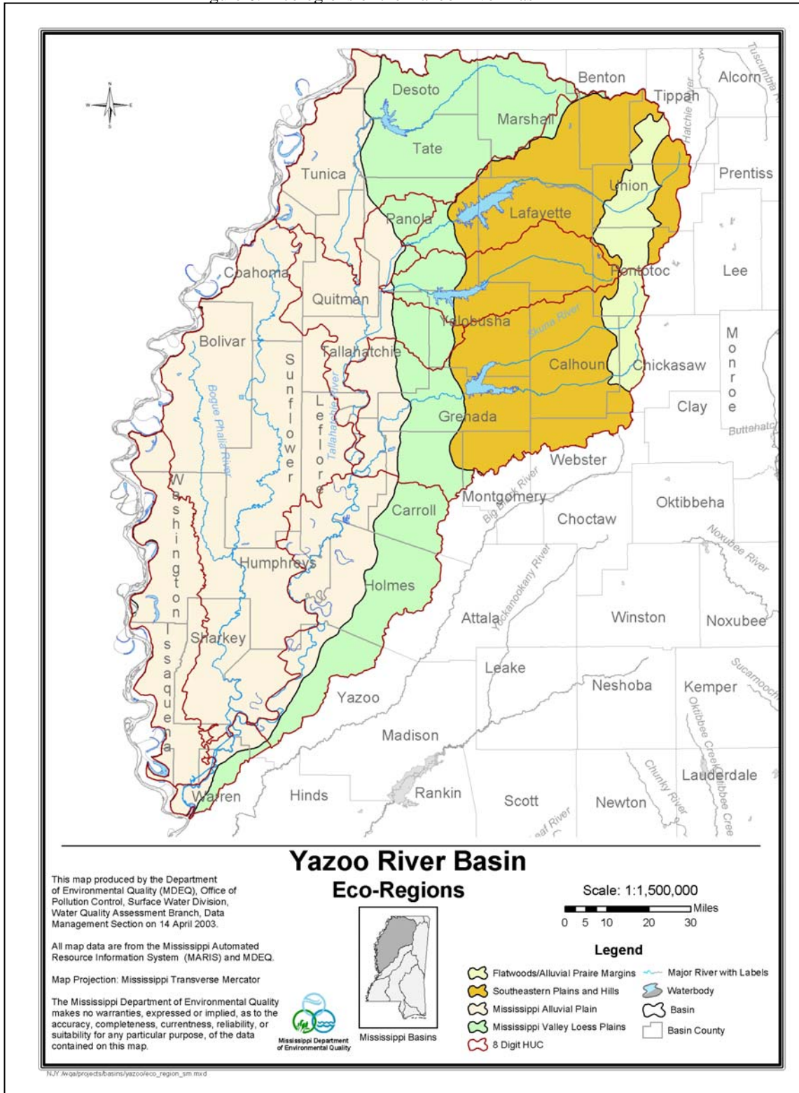
Figure 6. Ecoregions of the Yazoo River Basin
